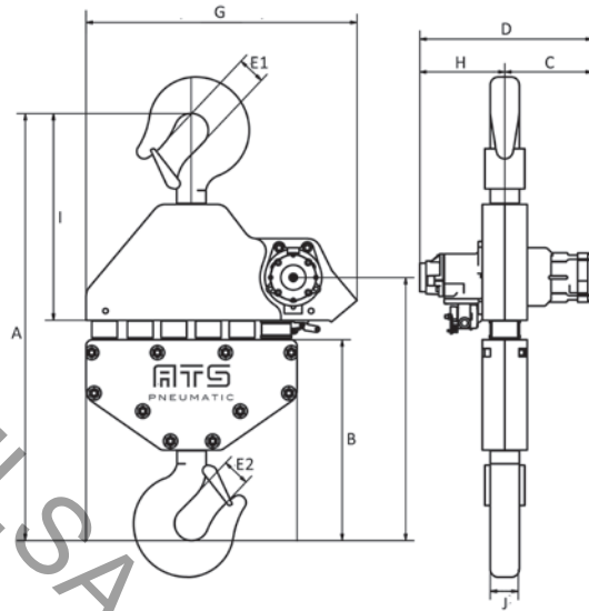
DIM. - ATS AIR CHAIN HOIST - 30ton - 37ton
